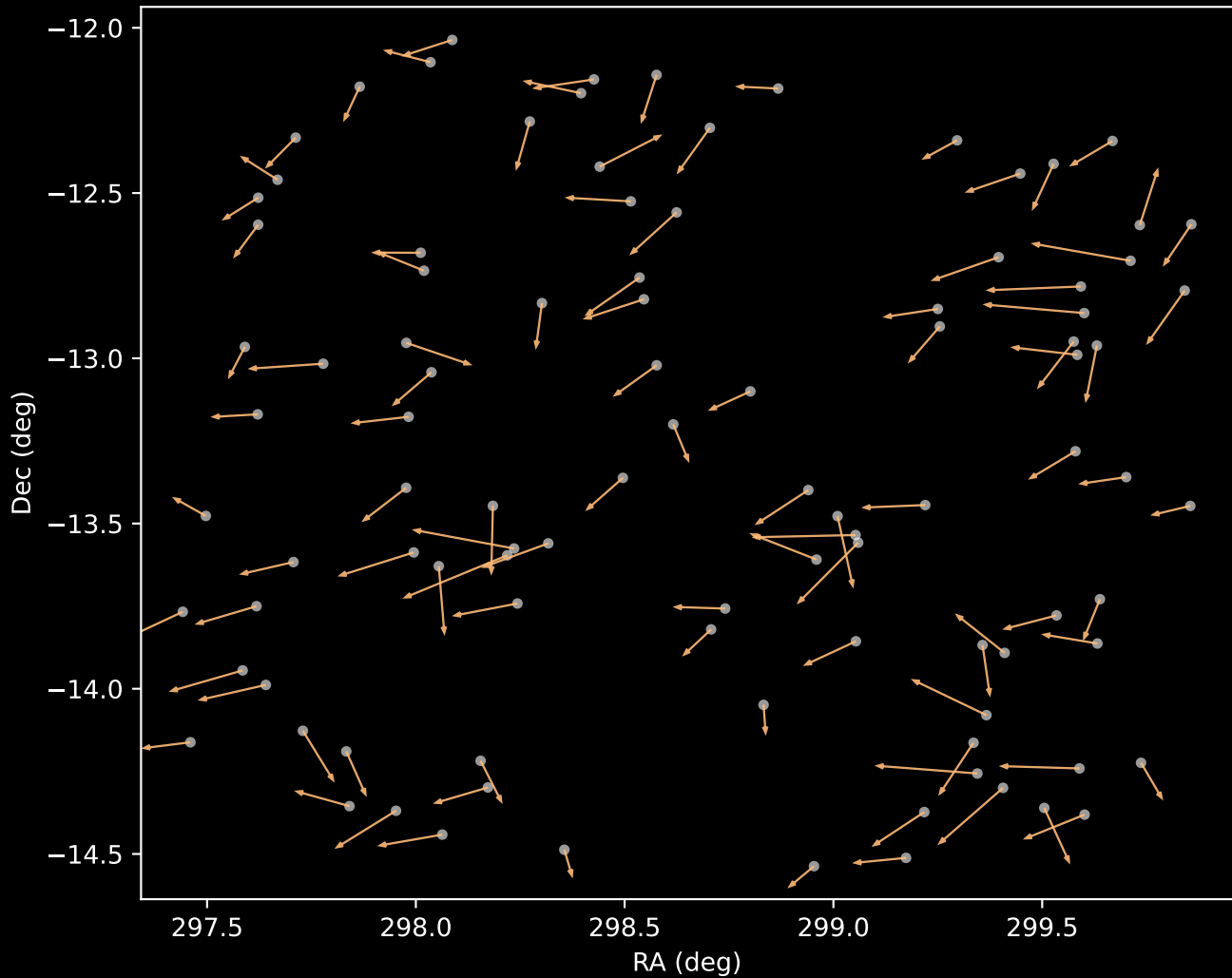
APOGEE DR17 Cluster 3 Proper Motion Vectors (n=99)
