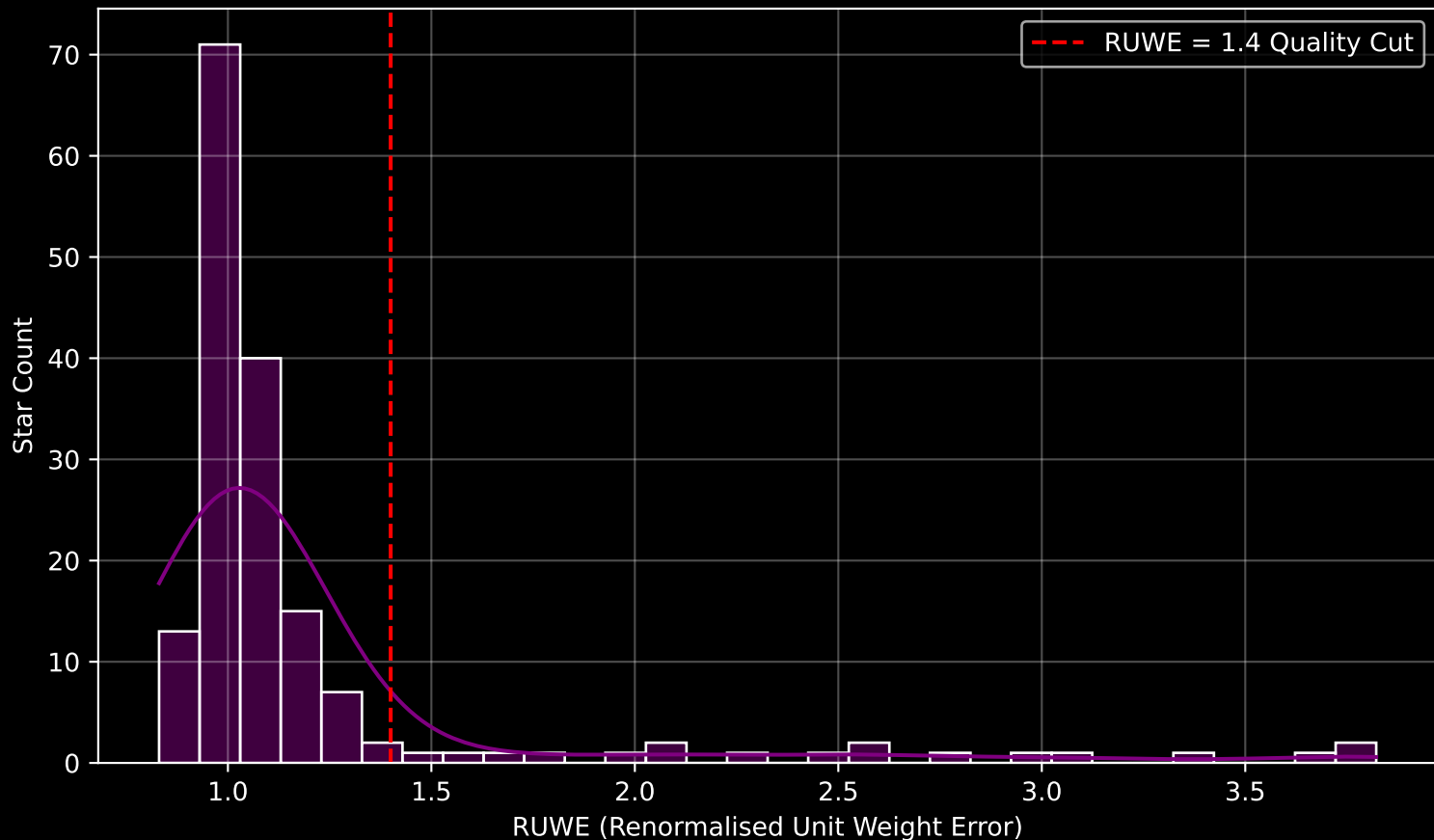
GAPOGEE DR17 Field [K2_C6_312+49_btx] RUWE Distribution (n= 166)
