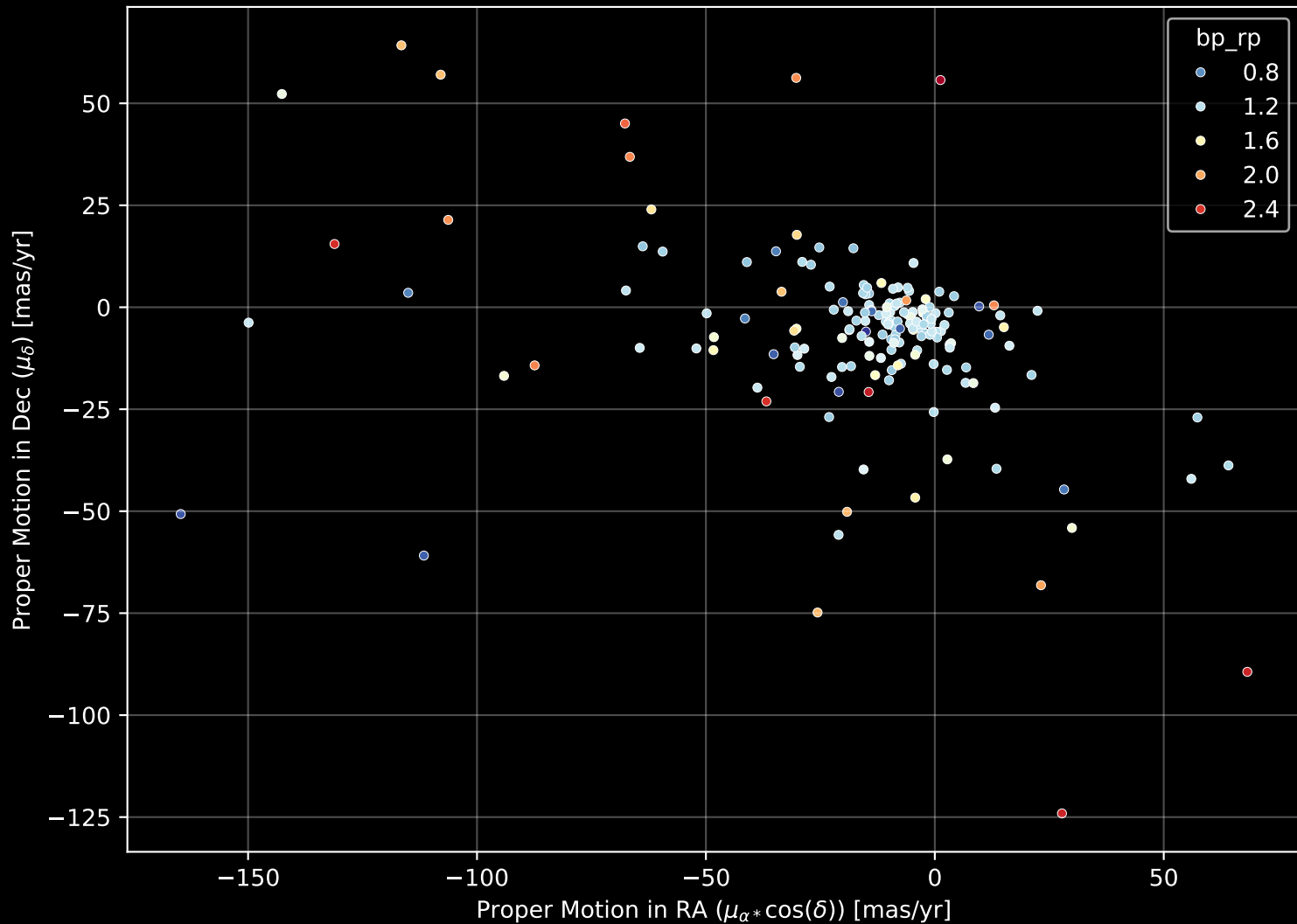
APOGEE DR17 Field: [K2_C6_312+49_btx] Proper Motion Diagram (n= 173)
