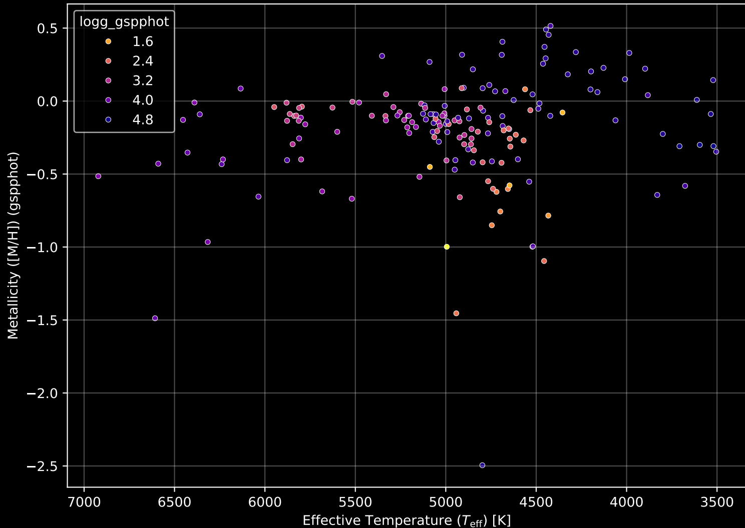
APOGEE DR17 Field: [K2_C6_312+49_btx] Stellar Population Parameters (n= 173)
