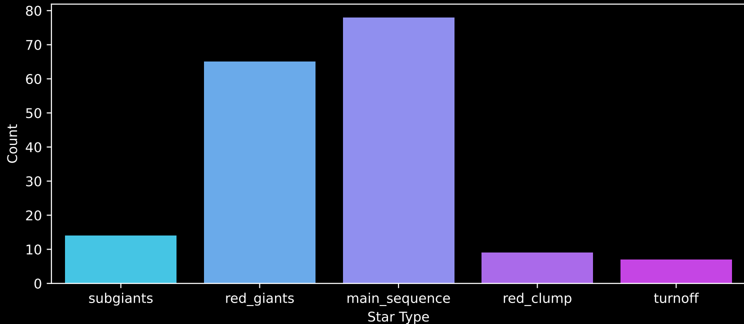
APOGEE DR17 Field: [K2_C6_312+49_btx] Count plot of Star Type
