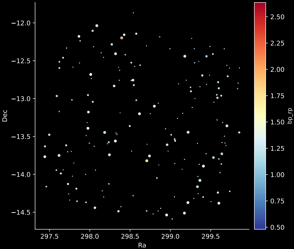
APOGEE DR17 Field: [K2_C6_312+49_btx] Stars: 173
