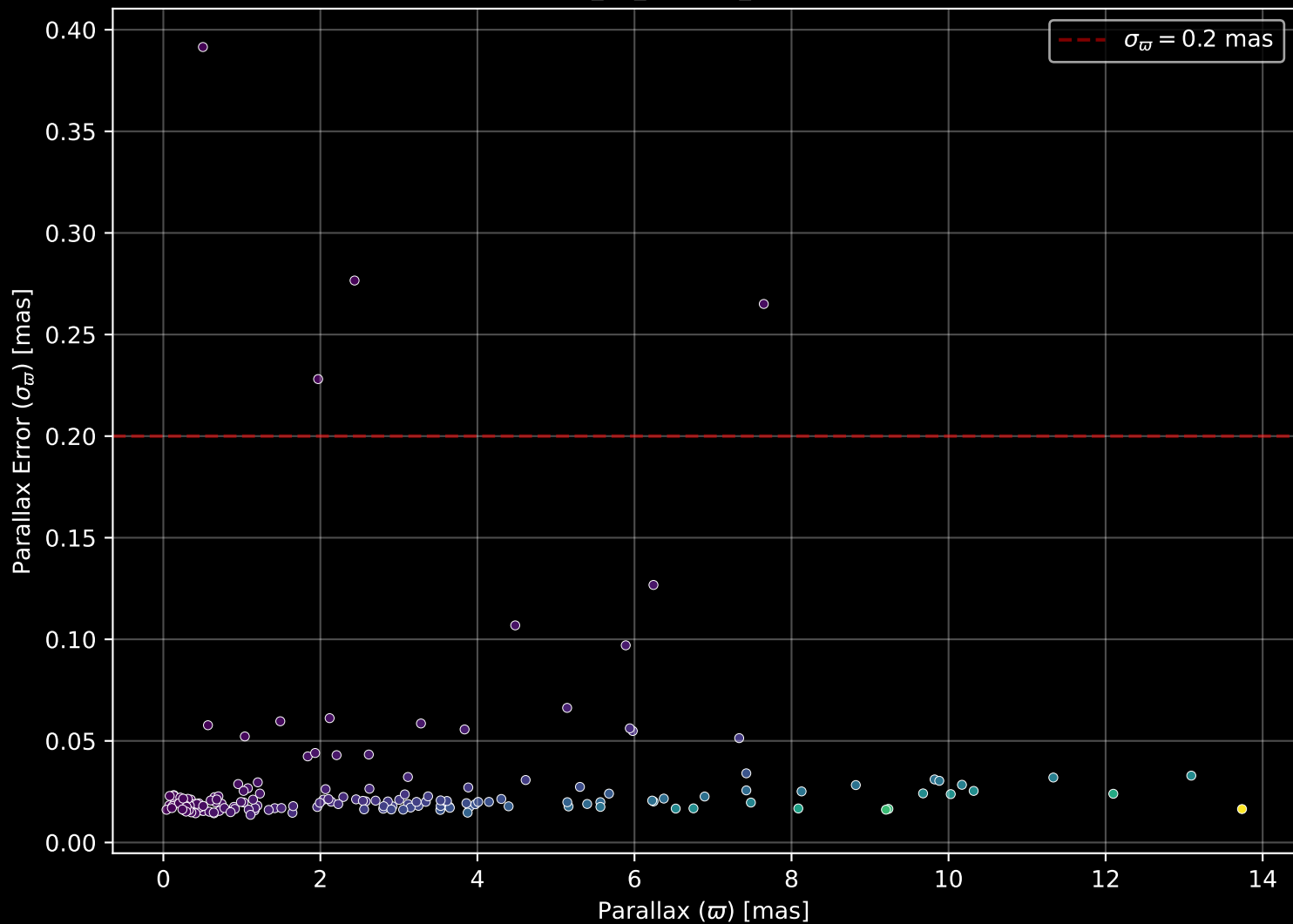
APOGEE DR17 Field: [K2_C6_312+49_btx] Parallax Quality (n= 173)
