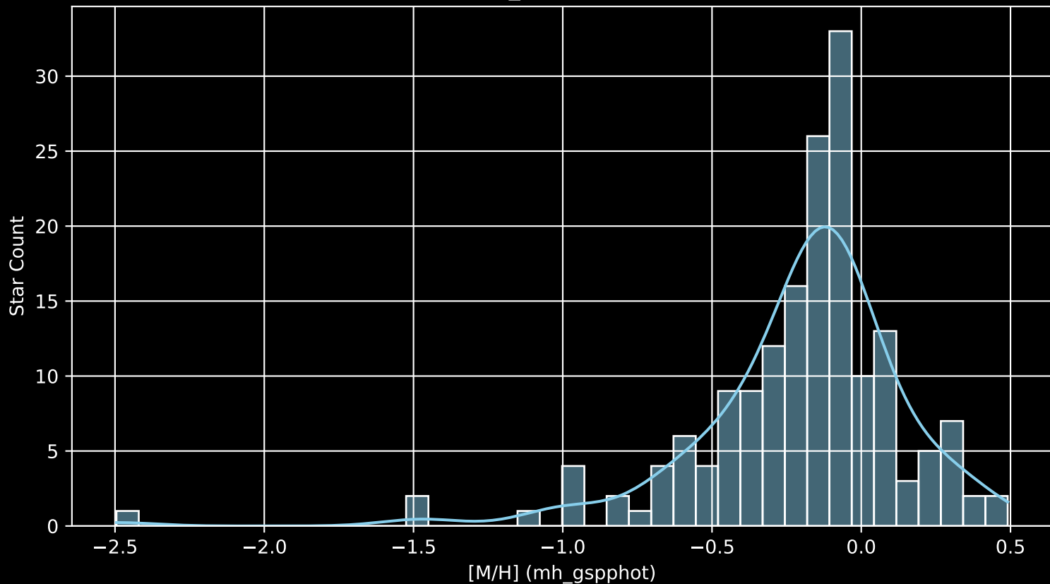
APOGEE DR17 Field: [K2_C6_312+49_btx [M/H] (mh_gspphot) (n= 172)
